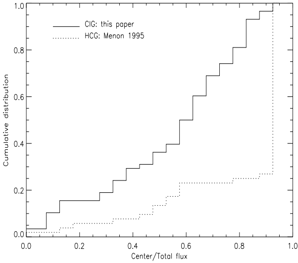
Fig. 11. Cumulative distribution of the FIRST/NVSS flux ratio for the CIG (solid line) and the center/total flux ratio (dotted line) from Menon (1995).
